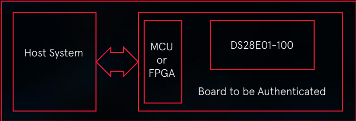
Figure 6 - A hardware authentication example using the DS28E01-100.
