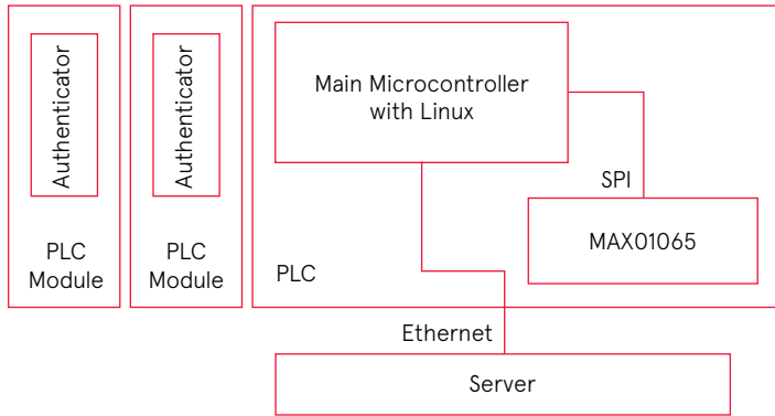
Figure 2 - Enabling security with PLC.
