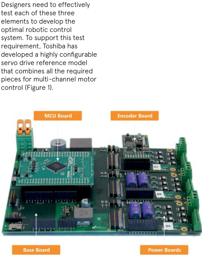
Figure 1 - Toshiba's servo drive reference model is highly modular, allowing a broad range of servo motor approaches to be trialled and implemented.
