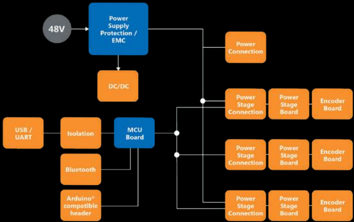
Figure 2 - The block diagram for Toshiba's servo drive reference model baseboard.
