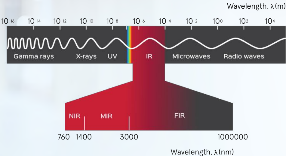
Figure 1 – The electromagnetic spectrum. Definitions are based on ISO21348 – Space environment (natural/artificial).
